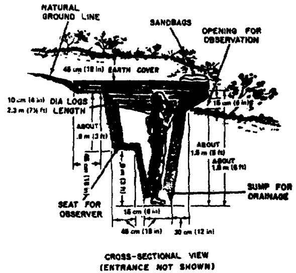
Figure 1-46. Observation post.
